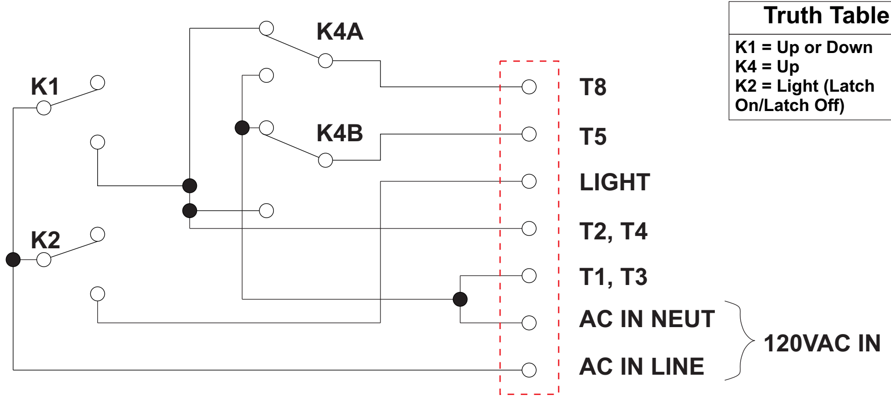
Relays shown in off position
