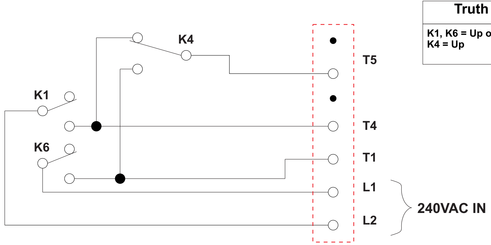
Relays shown in off position
