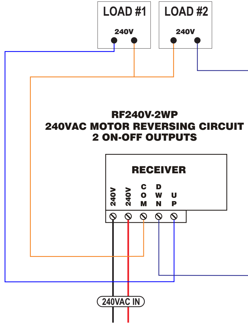
RF240V-2WP WIRING DIAGRAM
